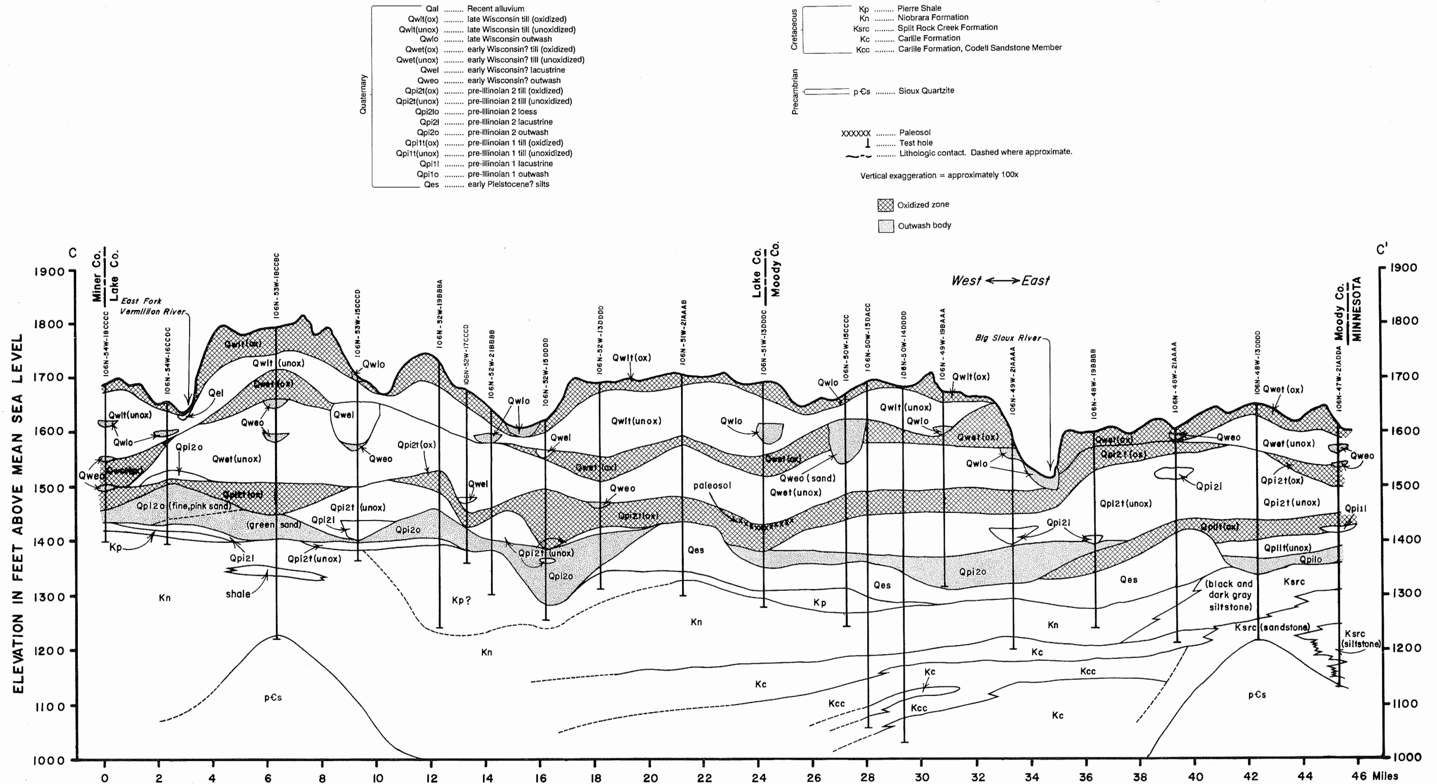
Figure 9. Geologic cross section C - C'. See Figure 6 for location.
