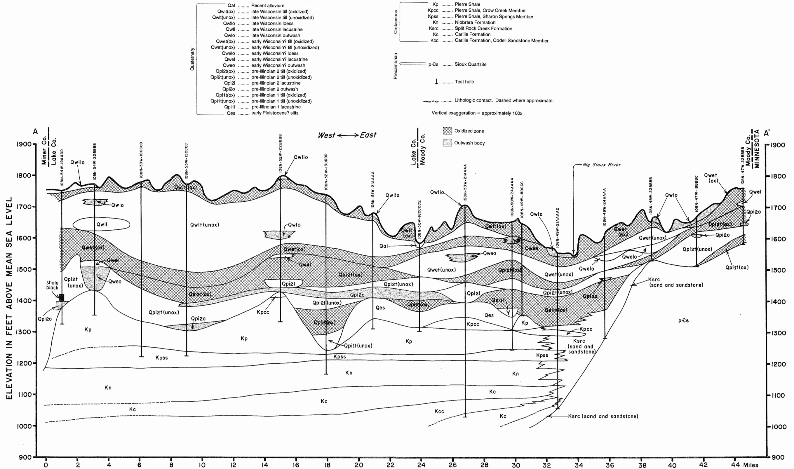
Figure 7. Geologic cross section A - A'. See Figure 6 for location.
